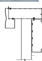
W-PAN TO C-BEAM TO POST
